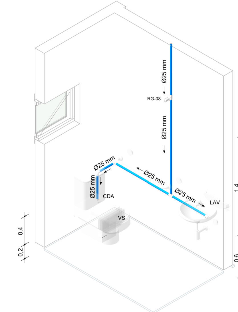
8 ISOMETRIA LAVABO PDC
